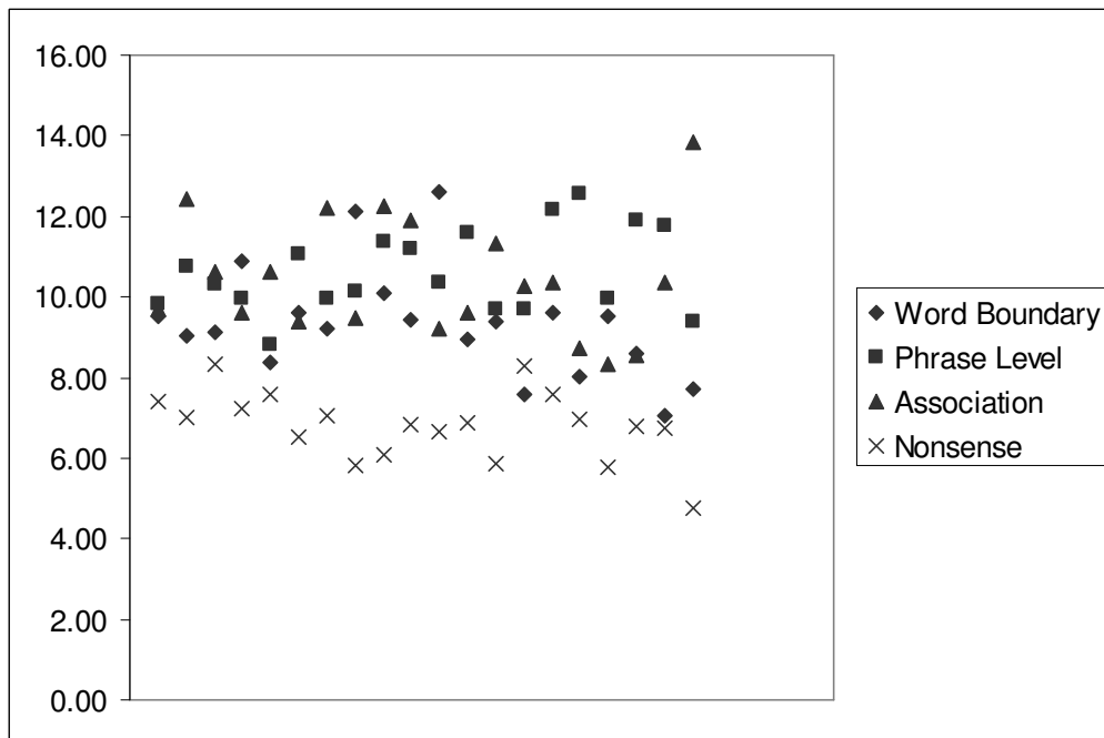
Fig 4: Scores for the positive and nonsense pairings using the average association ratio overlap leaving no clear dividing line (overlap is 14%).
