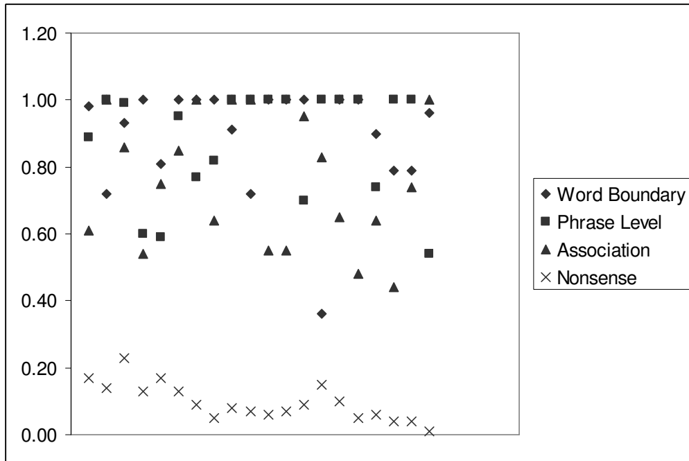
Fig 3: Scores for positive pairings and nonsense pairings using the Russian Doll algorithm fall into two discrete sets (overlap is 0%).
