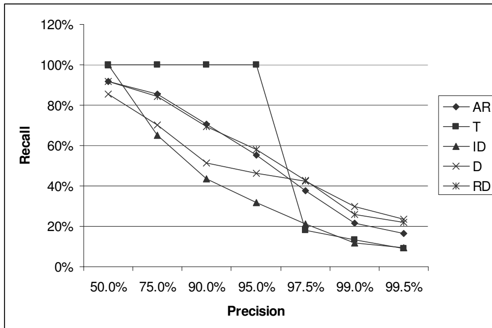
Fig 1: Recall vs Precision for the various measures.
